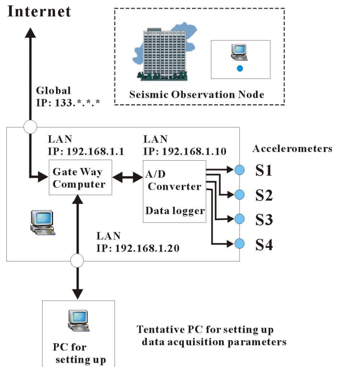
Constitution of Sensor Network for Seismic Observation
